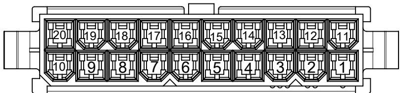
20 CKTS.
