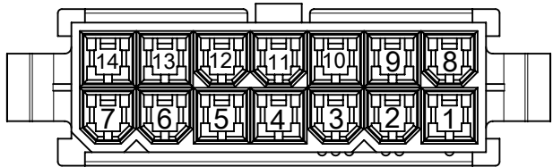
14 CKTS.
