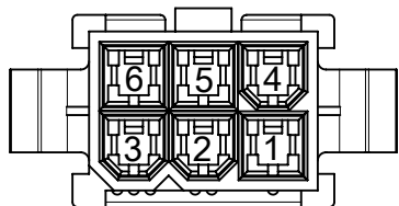
6 CKTS.
