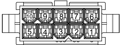
10 CKTS.
