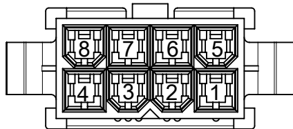
8 CKTS.
