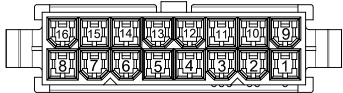
16 CKTS.
